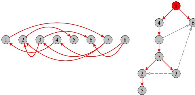
Fig. 1 Toy elements of law connected by reference edges (left) and a reference tree rooted at element 8 (right), where edges not in E_g are drawn as gray dashed arrows
